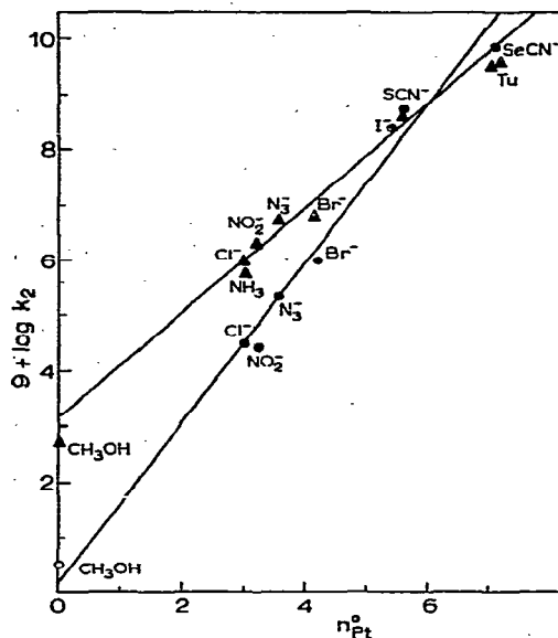
Fig. 1. Correlation between the rates of reaction of \text{Pt}^{\text{II}} complexes in methanol at 30 °C with the standard \text{trans-}[\text{Pt}(\text{pyridine})_2\text{Cl}_2] for different entering groups: \text{trans-}[\text{Pt}(\text{PEt}_3)_2\text{Cl}_2] ●; \text{trans-}[\text{Pt}(\text{piperidine})_2\text{Cl}_2] ▲.
